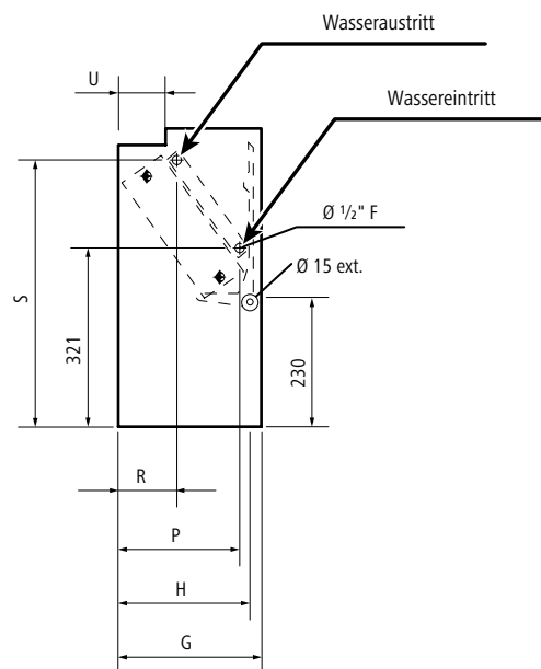
4-Leiter Systeme
