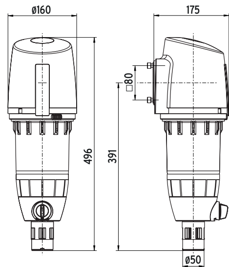
Maße [mm]
