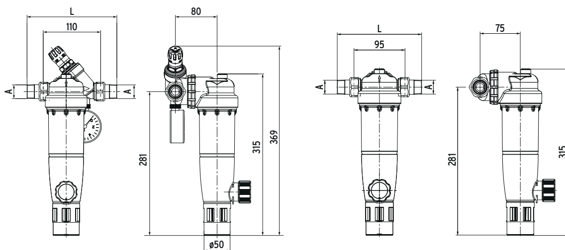
Maße [mm]
